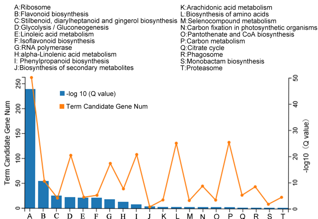
Fig. S5. Function enrichment analysis of DEGs in the tuberous roots (mixture of ITRs+MTRs +LTRs) (TRs) compared to UFRs.
